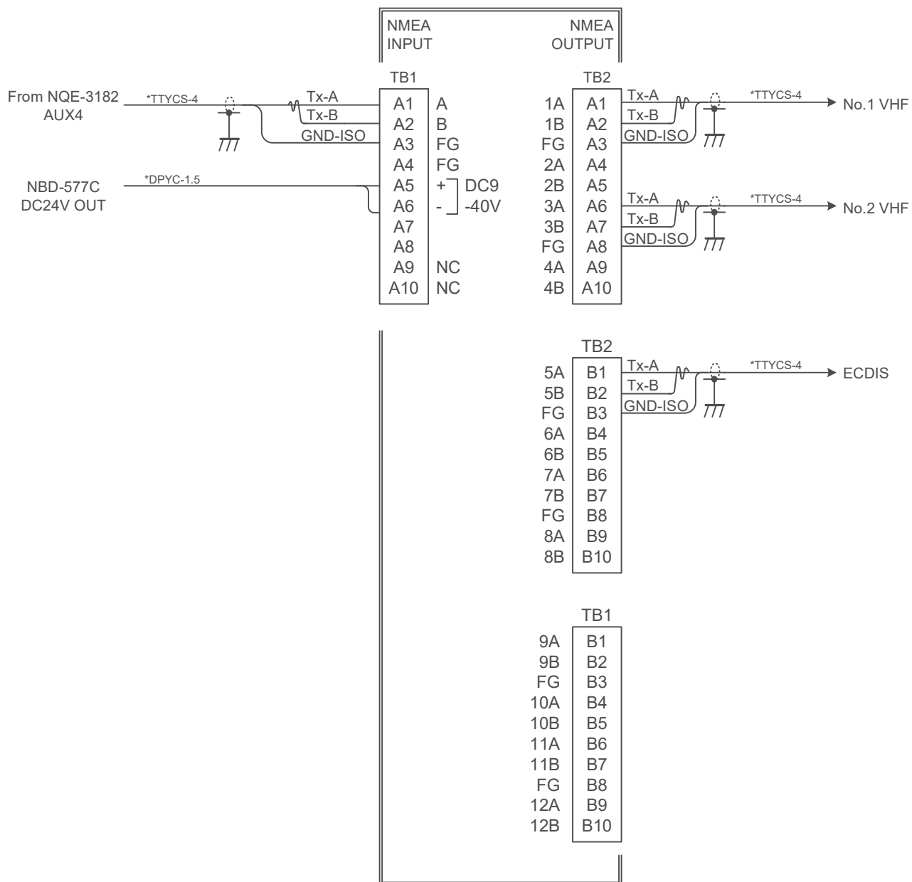
NQA-4251 BUFFER UNIT
