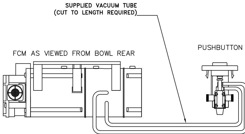
DETAILS OF VACUUM TUBING INSTALLATION
