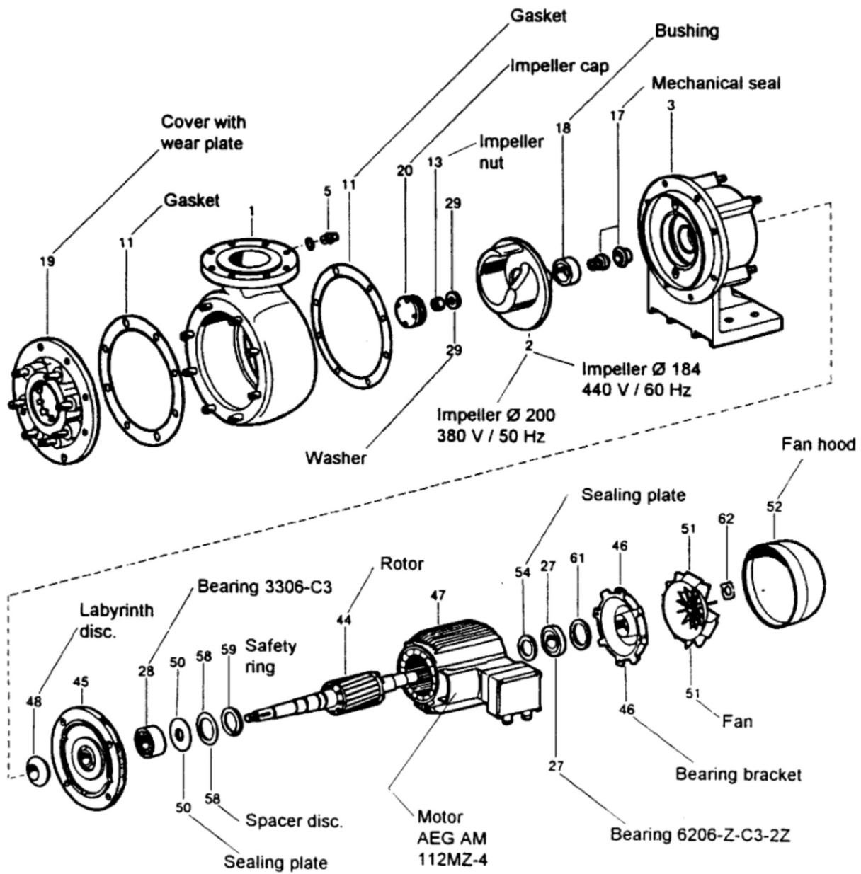
Figure 5.1 Pump Type 5,5 QSH 101-F
